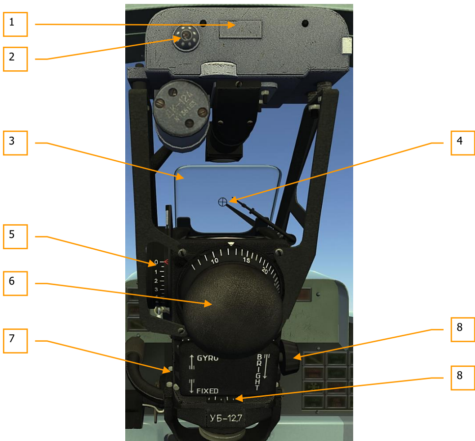
Figure 158: ASP-3NMU gunsight and FKP-2-2 guncamera
