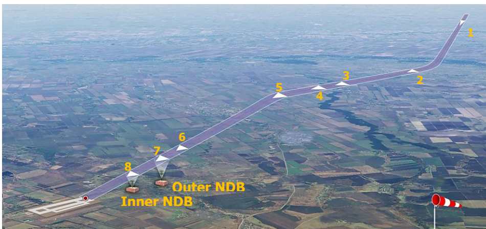
Figure 153: Landing pattern using GLIDE PATH and LANDING modes
