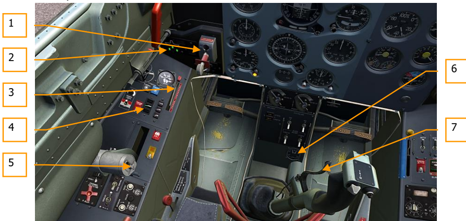
Figure 51: Utility hydraulic system controls and indication, rear cockpit
