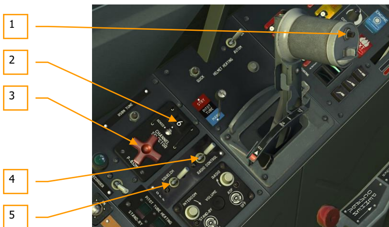
Figure 128: R-832M controls
