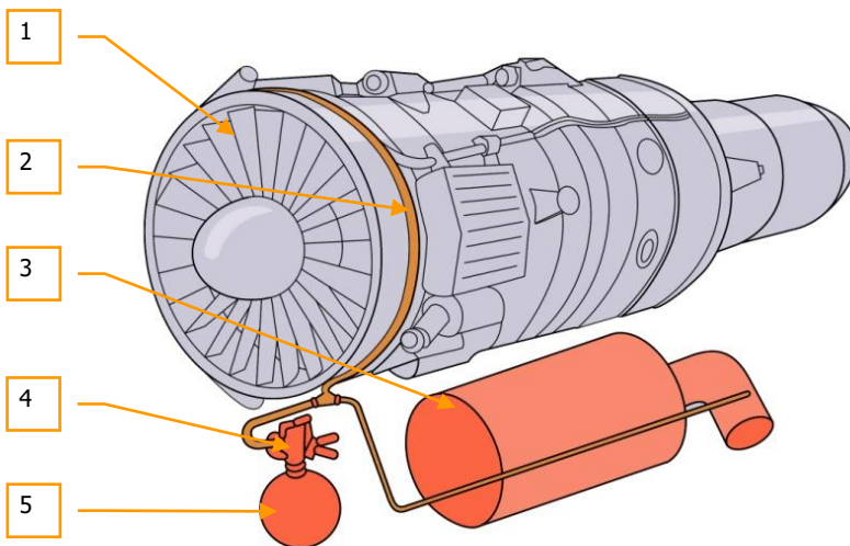
Figure 66: Engine fire extinguishing equipment
