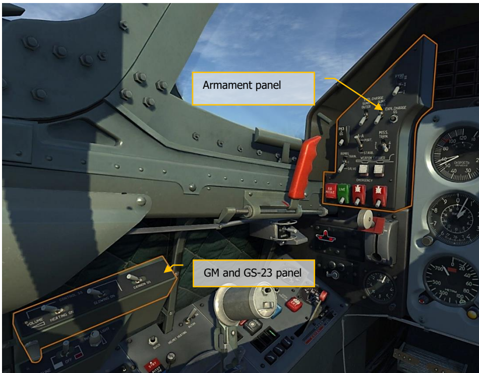
Figure 167: Armament control panels
