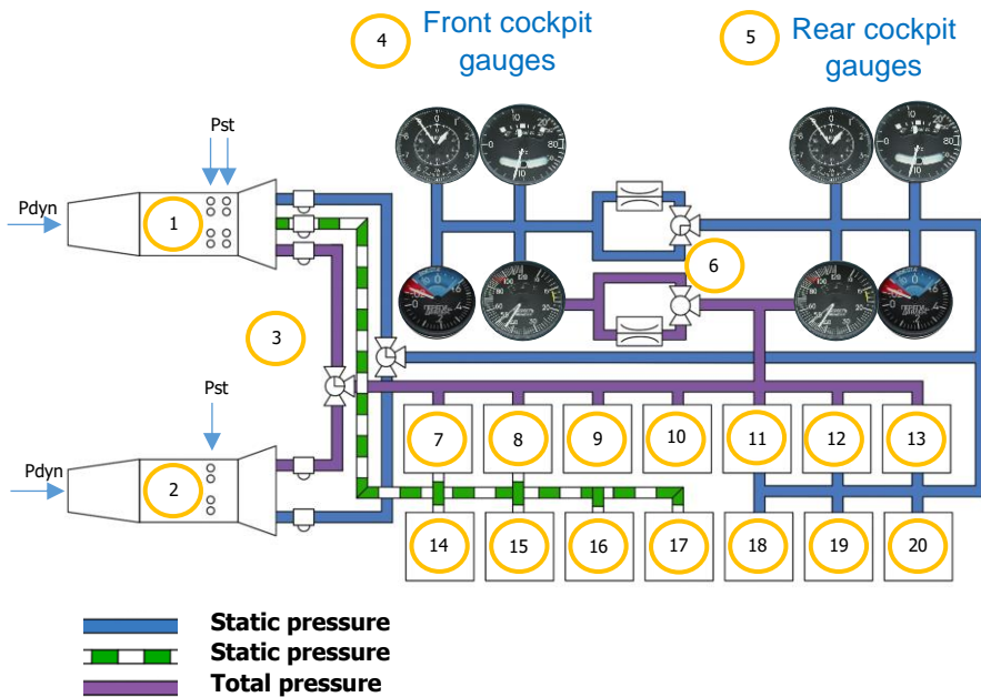
Figure 106: Pitot-static system
