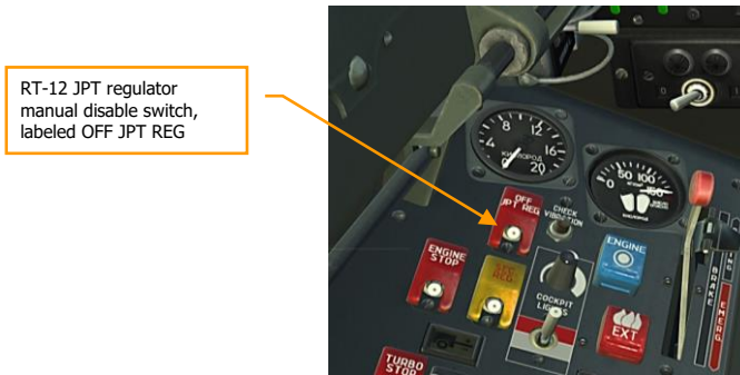
Figure 75: RT-12 JPT regulator manual disable switch
