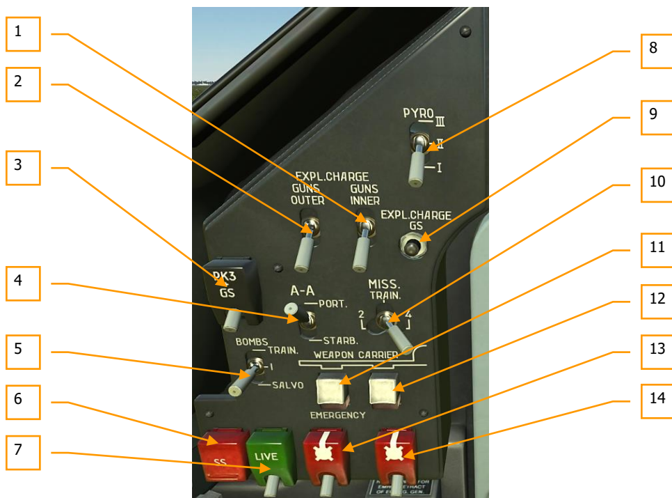
Figure 182: Armament panel
