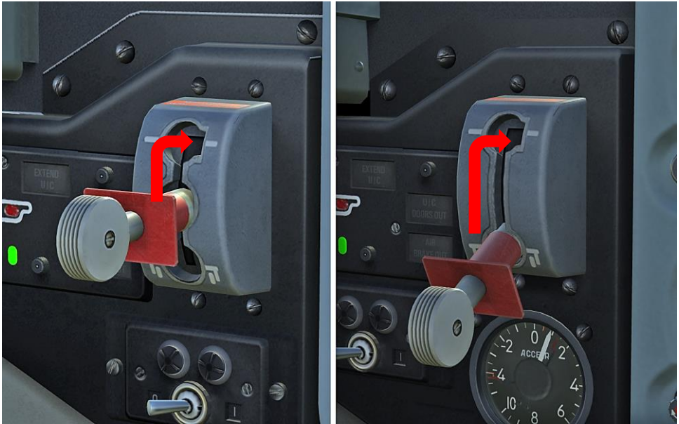
Figure 54: Emergency gear retraction, rear (left) and front (right) cockpit
