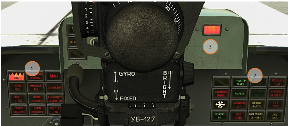
Figure 95: Warning lights and caution & advisory lights panels, front cockpit
