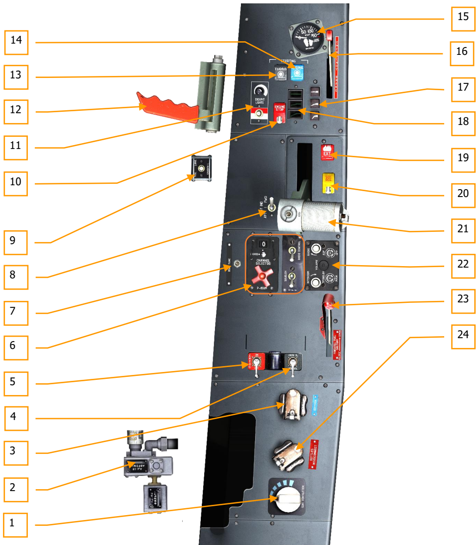
Figure 104: Rear cockpit, left panel
