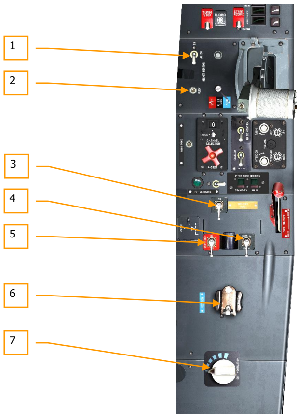
Figure 125: KKO-5 controls on the left panel in front cockpit
