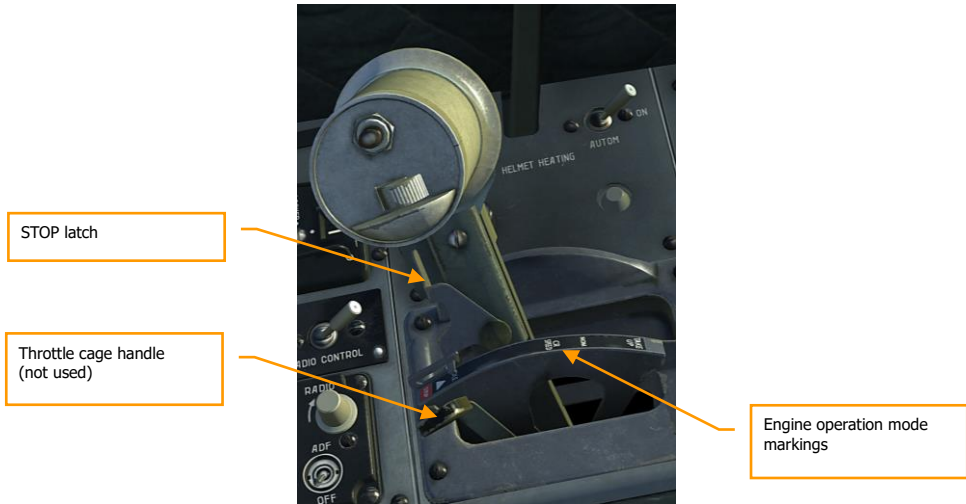
Figure 79: Throttle, front cockpit
