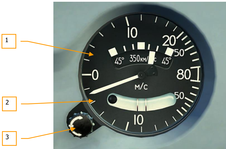
Figure 112: Combined gauge variometer
