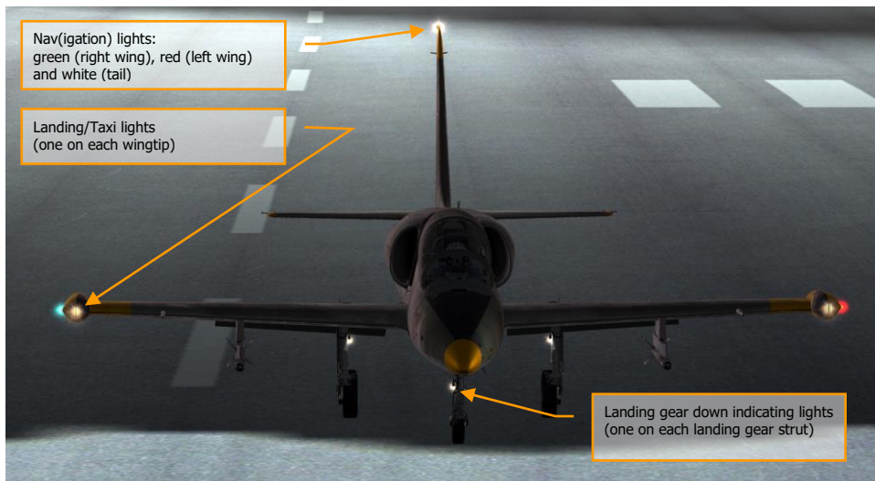
Figure 88: Exterior lights
