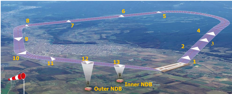
Figure 150: Circle pattern flight
