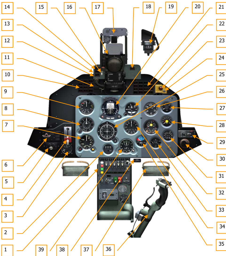
Figure 99: Front cockpit, central panel
