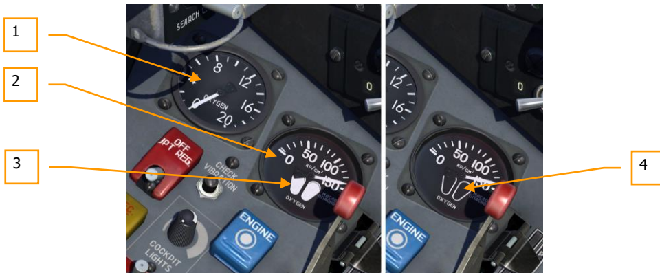
Figure 124: KKO-5 controls
