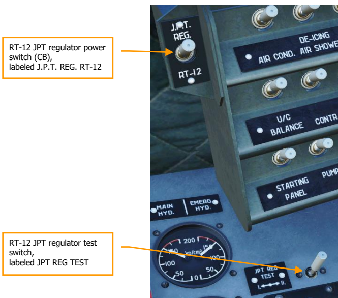
Figure 76: RT-12 JPT regulator power and test switches
