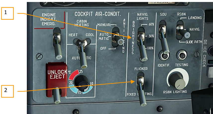
Figure 89: Controls for navigation lights
