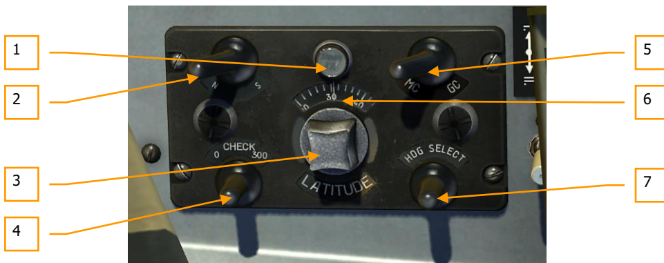
Figure 122: PU-26E control panel
