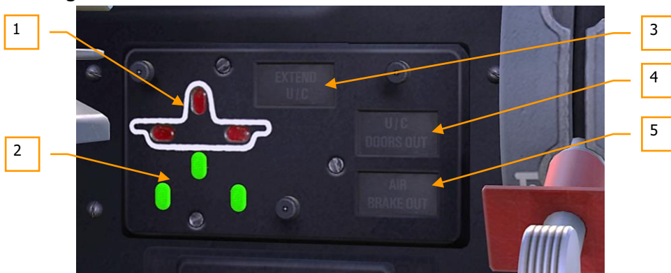
Figure 52: Landing gear position indicator panel
