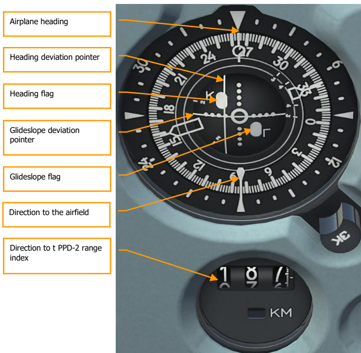
Figure 152: RMI
