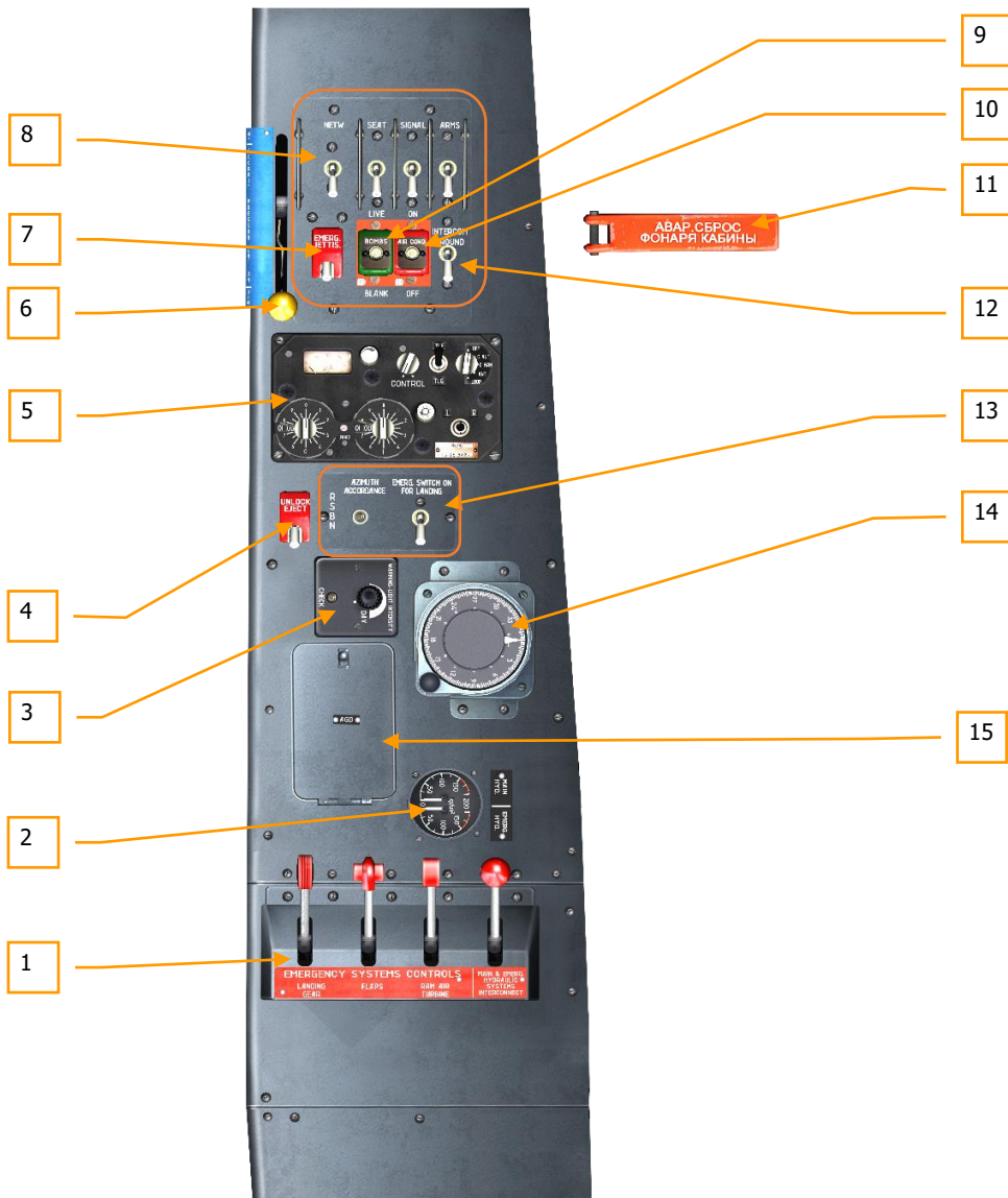
Figure 105: Rear cockpit, right panel
