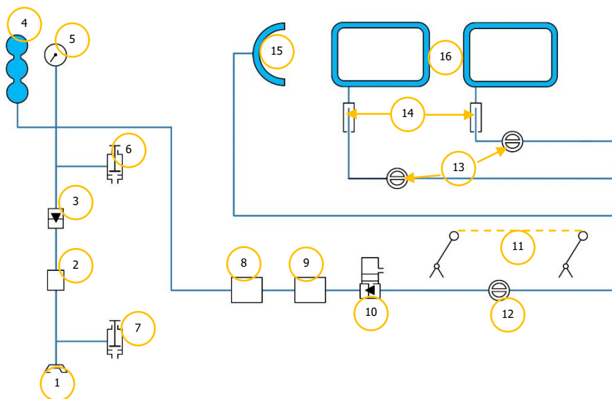
Figure 59: Environmental control system diagram
