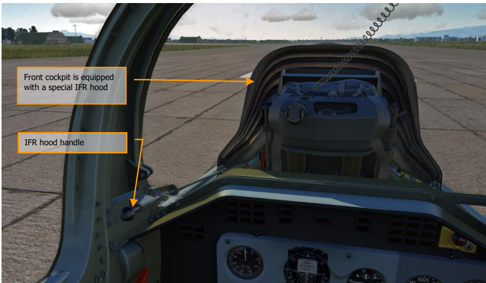
Figure 41: Lowered IFR hood, rear cockpit view
