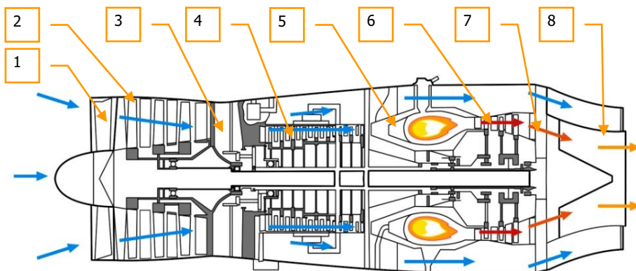
Figure 71: AI-25TL engine
