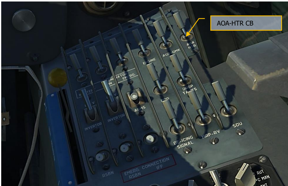
Figure 179: The AOA-HTR CB on the main switch panel
