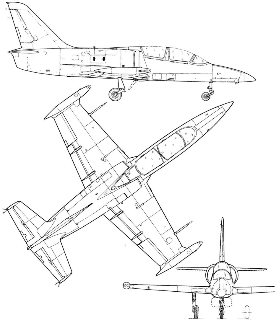
Figure 33: L-39 drawings
