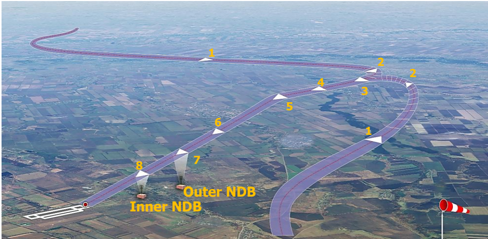
Figure 154: Scheme of airfield approaching and landing approach using LANDING mode
