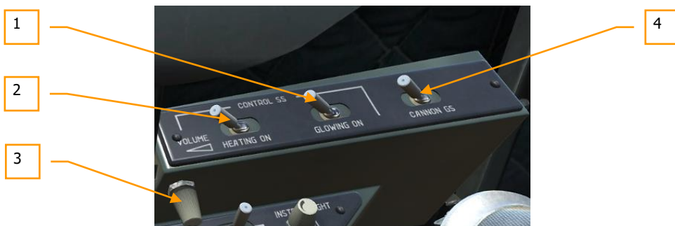
Figure 184: R-3S, R-60 and GS-23 Control Panel
