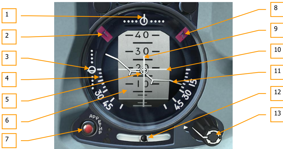
Figure 113: KPP-1273K ADI
