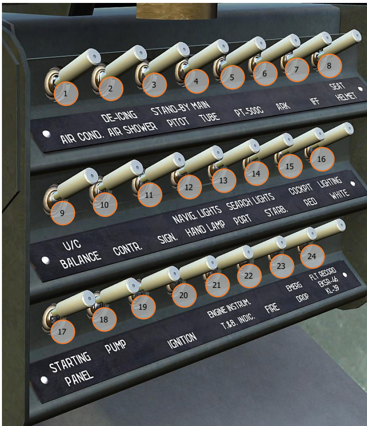
Figure 85: Auxiliary electrical CB panel, front cockpit
