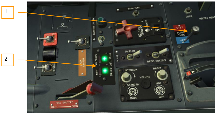
Figure 107: Pitot-static system controls
