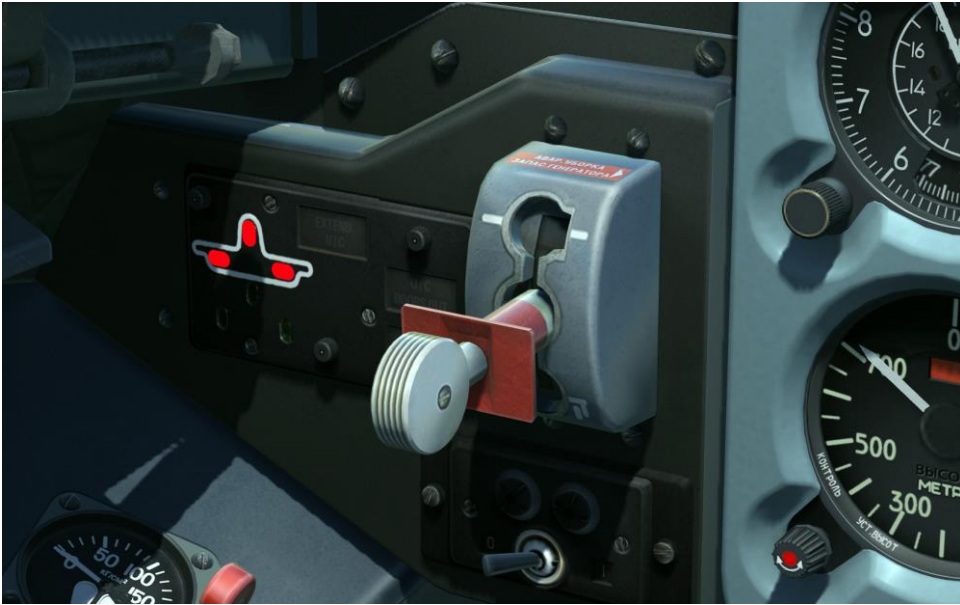
Figure 46: Landing gear lever, rear cockpit
