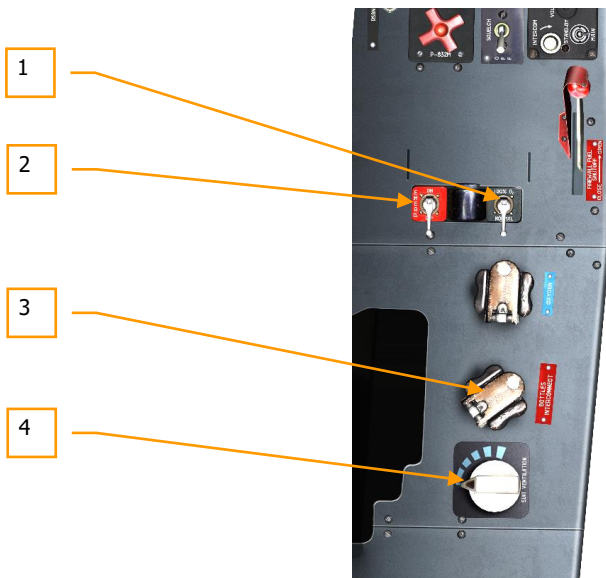
Figure 126: KKO-5 controls on the left panel in rear cockpit
