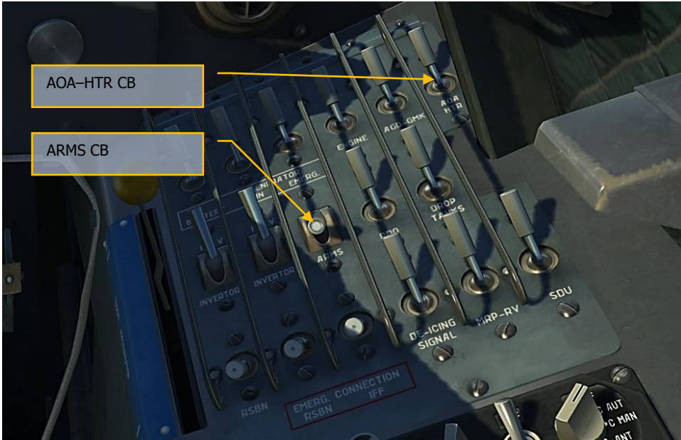
Figure 171: Main switch panel
