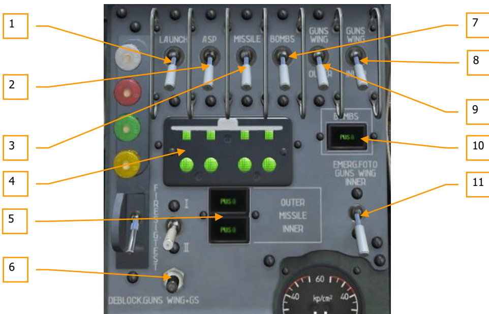
Figure 183: Center Panel
