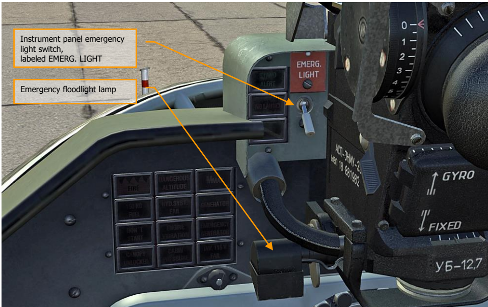
Figure 93: Instrument panel emergency light
