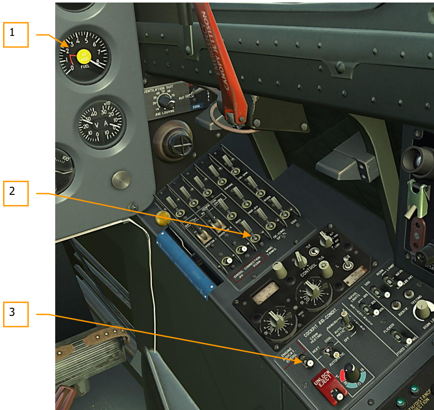
Figure 65: Fuel management controls
