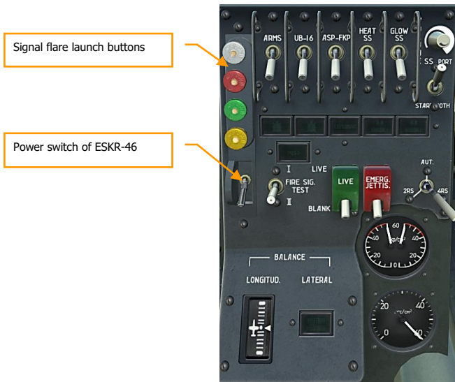
Figure 162: EKS-46 control panel
