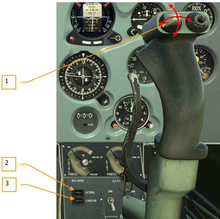
Figure 58: Trimmer controls, rear cockpit
