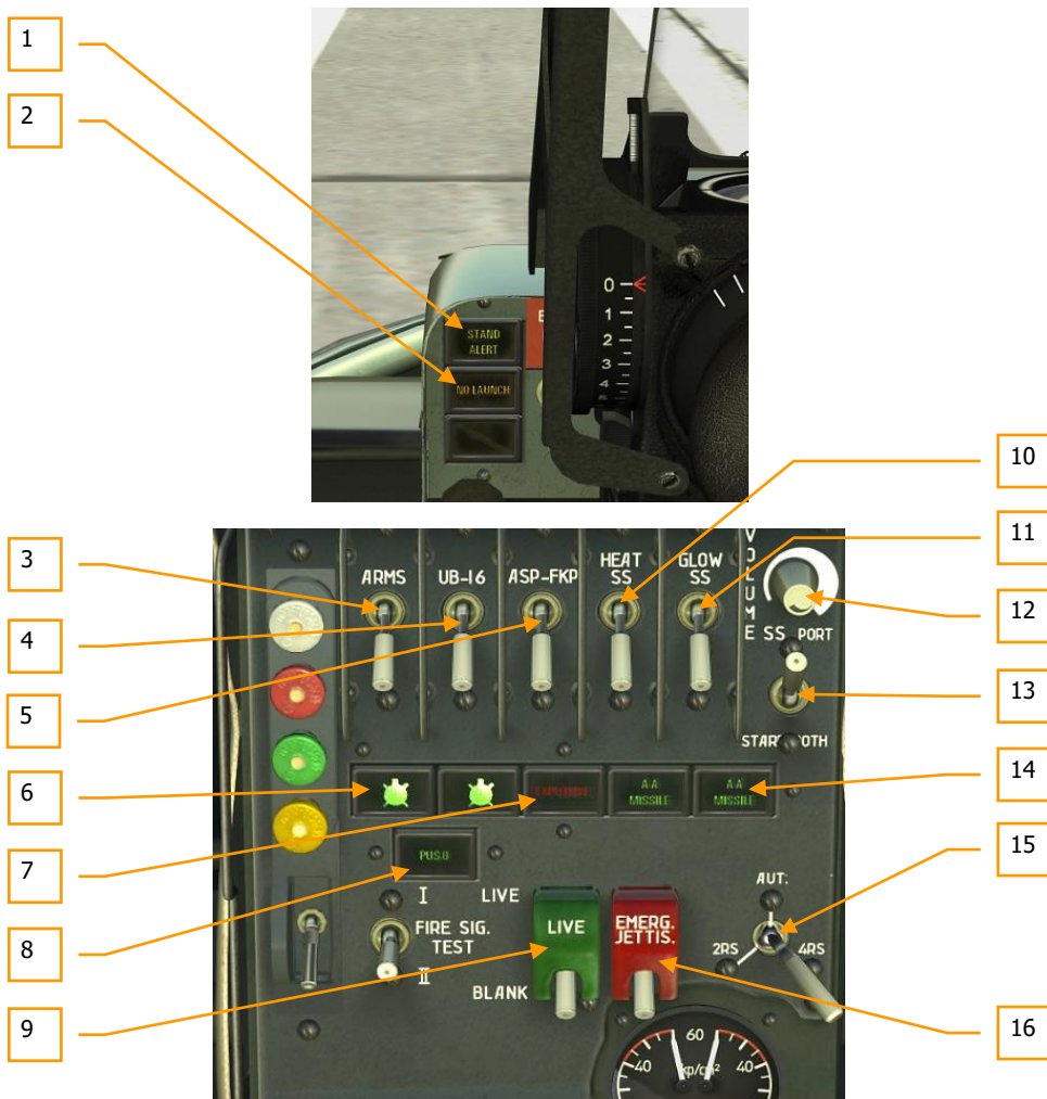
Figure 156: Armament controls and signalization in front cockpit
