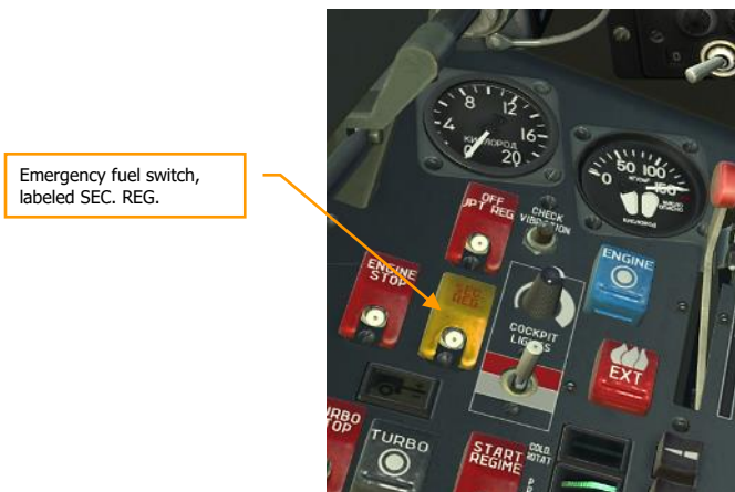
Figure 73: Emergency fuel switch
