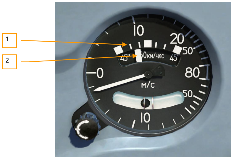
Figure 115: Turn and slip indicator
