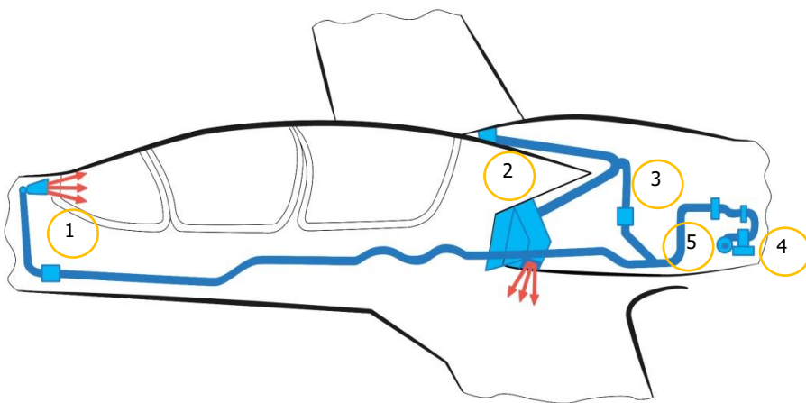
Figure 69: Anti-icing system
