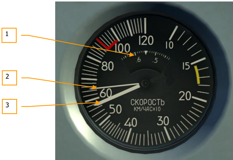
Figure 111: KUSM-1200 airspeed and Mach number indicator
