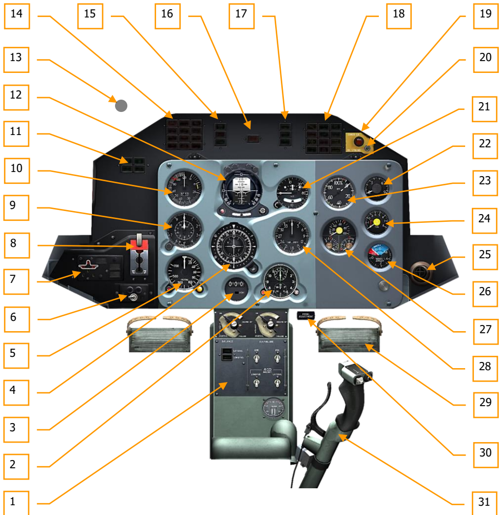
Figure 103: Rear cockpit, front panel
