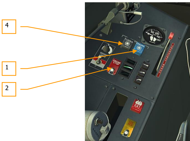
Figure 78: Engine controls, rear cockpit
