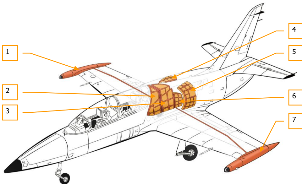
Figure 63: Fuel tanks
