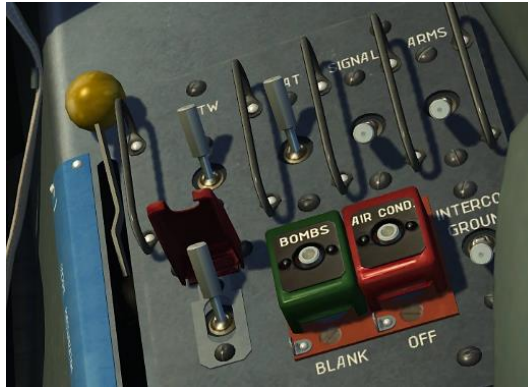
Figure 178: The EMERG. JETTIS. switch in the rear cockpit
