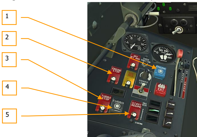
Figure 77: Engine controls, front cockpit
