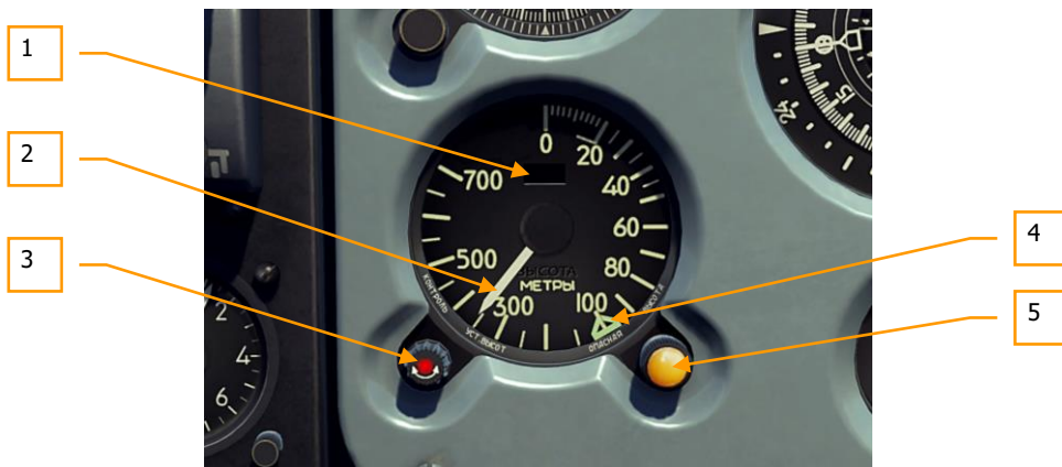
Figure 140: RV-5 Low Altitude Radar Altimeter
