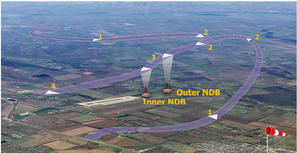
Figure 155: Landing scheme with help of RKL-41
